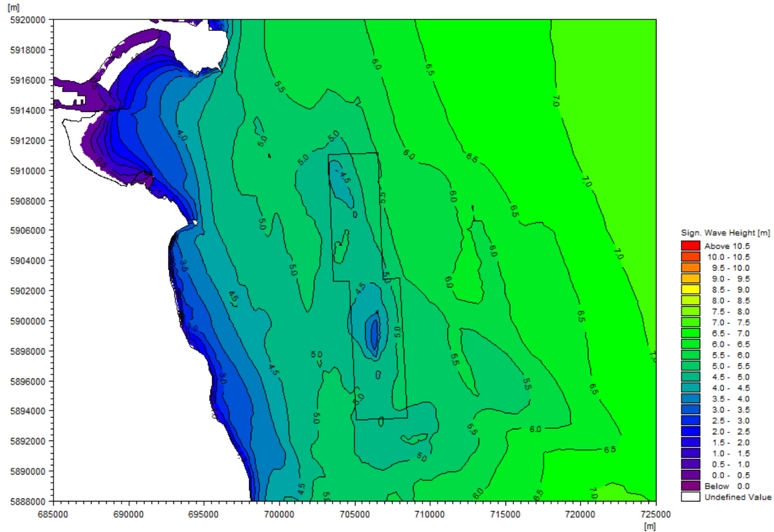
Figure 4 Significant wave heights from the south (a 1 in 1 year event) (DAPPMS)
